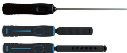
Smart air temperature probe with 2 m cable - Ref. 24646
